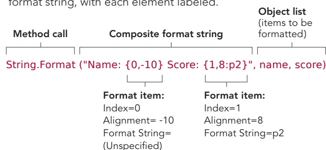
Figure 1. The anatomy of a call to String.Format
