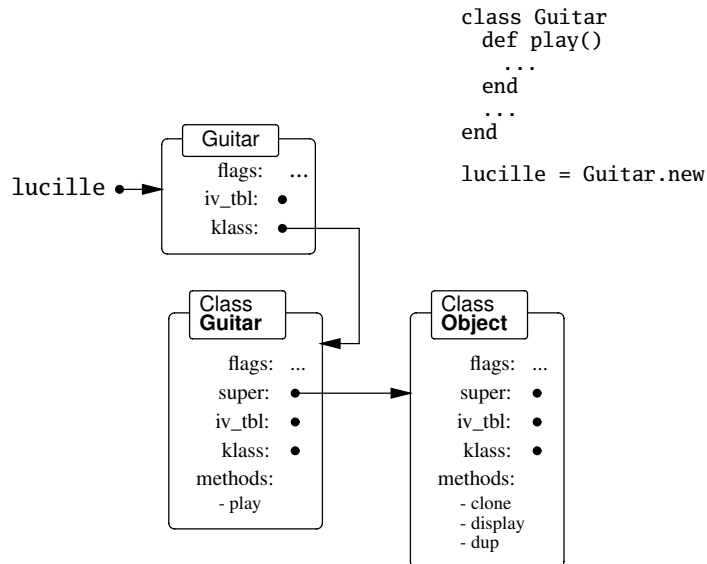
Figure 24.1. A basic object, with its class and superclass
