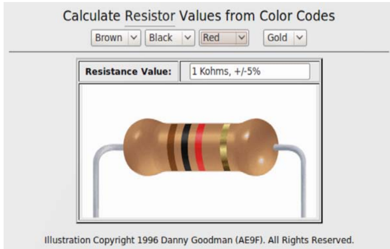
Figure 1-7. This screen-shot shows the web application designed by Danny Goodman. I have this web page bookmarked in my web browser and use it often to check unfamiliar resistor color codes.
