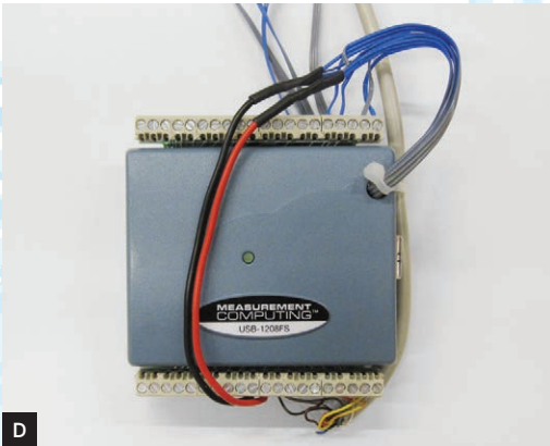
A0–A4 (terminals 21–25) respectively, and pin 7 of the cable to digital port A7 (terminal 28), as shown in Figure D.
