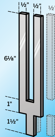
Tuning Fork Layout Diagram
