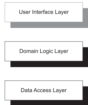
Figure 2.7 At this point, Mary has implemented the Data Access Layer and the Domain Logic Layer. Compared to figure 2.6, the Domain Logic Layer has been added. The User Interface Layer still remains to be implemented.
