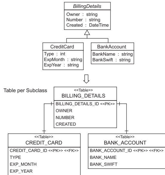
Figure 3.11 Table-per-subclass mapping
